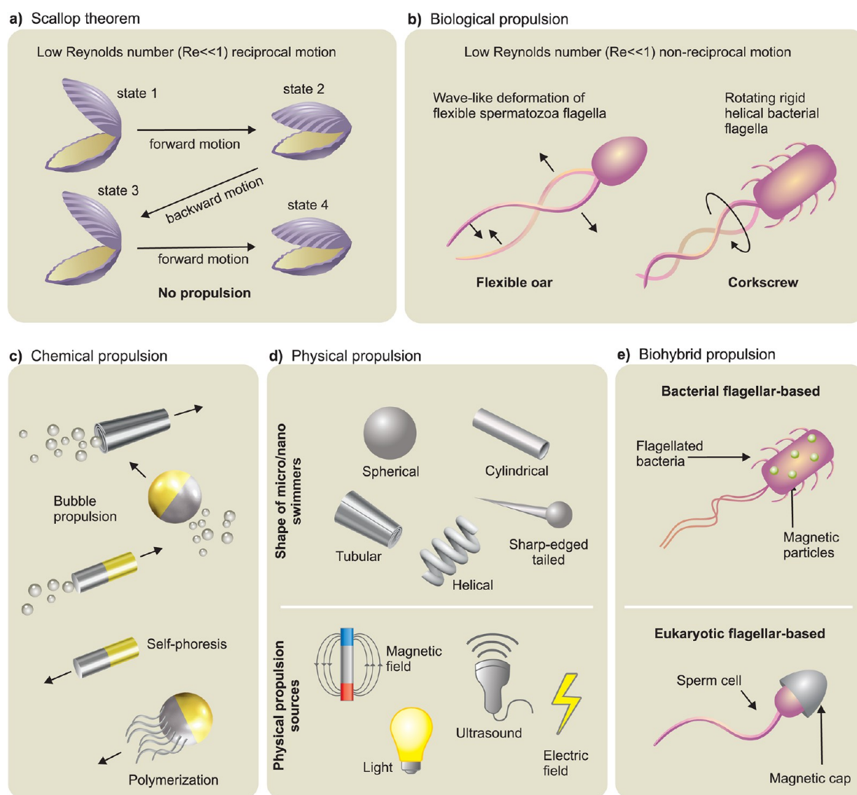
Figure 2. Theory of locomotion at low Reynolds numbers and micro/nanorobot propulsion mechanisms. a) Schematic drawing of Purcell's "Scallop Theorem" with reciprocal motion at low Reynolds number regime. Adapted from ref 161, Copyright 1977 AIP Publishing. b) Two main biological propulsion mechanisms based on nonreciprocal motion at low Reynolds number regime, i.e. , beating a flexible oar (in eukaryotic flagellar-based propulsion) and rotating a chiral flagellum (in bacterial flagellar-based propulsion). Adapted from ref 161, Copyright 1977 AIP Publishing. c) Schematic overview of various chemical propulsion mechanisms utilized for different kinds of micro/nanomotors. d) Schematic overview of various kinds of micro/nanorobots propelled via external physical power sources, i.e. , magnetic field, acoustic field, light, and electric field. e) Schematic overview of biohybrid propulsion mechanisms based on prokaryotic (bacterial) and eukaryotic flagella.
