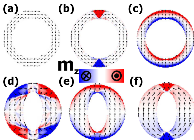
FIG. 3. Micromagnetic simulation of 10 \mu\text{m} rings with a 7 \mu\text{m} concentric circular aperture (a) initialized in a vortex state, (b) under 50 mT vertical field after (a), and (c) under 100 mT vertical field after (b). Ring with an elliptical aperture (7 \mu\text{m} × 3.5 \mu\text{m} ) (d) initialized in an anti-vortex state, (e) under 10 mT vertical field after (d), and (f) under 100 mT vertical field after (e). Arrows correspond to the planar magnetization and color coding reflects the out-of-plane magnetization component.
