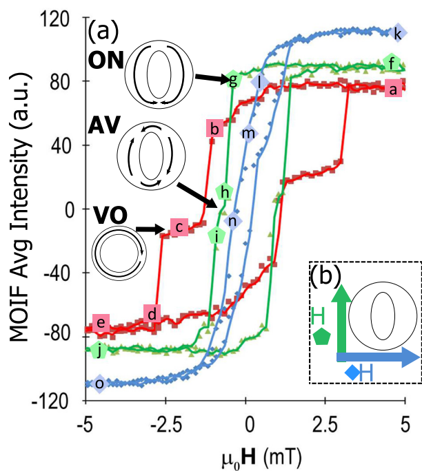
FIG. 1. (a) MOIF magnetization versus applied external field for 10\ \mu\text{m} rings with either a 7\ \mu\text{m} concentric circular hole (red squares and solid line), an elliptical hole with field applied along the 7\ \mu\text{m} long axis (green triangles/pentagons and solid line), or an elliptical hole with field applied along the 3.5\ \mu\text{m} short axis (blue diamonds and solid line). Magnetization configurations of the ring corresponding to an onion state (ON), a vortex state (VO), and an anti-vortex state (AV) are shown schematically. (b) Orientation of applied field with respect to ellipse axes.
