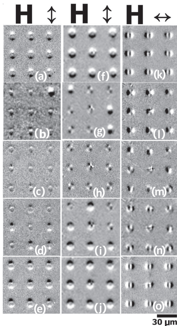
FIG. 2. MOIF images during remagnetization: circular hole with vertical field (a)–(e); (f)–(j) elliptical hole with vertical field; and (k)–(o) elliptical hole with horizontal field. Subfigures (a)–(o) correspond to fields along magnetization versus applied field data shown in Fig. 1.
