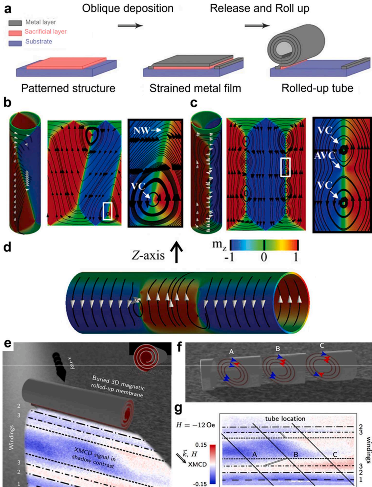
Fig. 5. Magnetic Domain Characteristics in Rolled-up Architectures. a, Schematic illustration of the device used for investigating magnetic domain structures in rolled-up tubular architectures. b, Random distribution and c, A predefined two-domain state of rolled-up permalloy domain structures. d, Domain structures of rolled-up nickel films. e, XMCD characterization of magnetic materials within tubular structures. f, XMCD images of different windings in the rolled-up system under varying external magnetic fields. g, Corresponding magnetic domain patterns. Reproduced with permission. Copyright © 2013, Wiley-VCH. Copyright © 2014, American Chemical Society.
