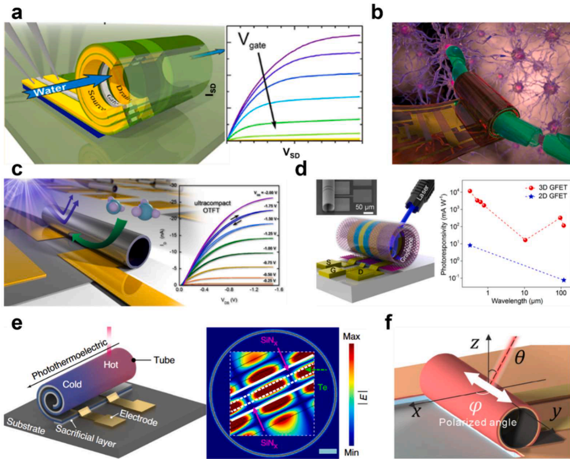
Fig. 3. Rolled-up active device. a, Schematic of the rolled-up transistor for microfluidics (left) and its electrical response (right). b, Schematic of the rolled-up Biomimetic microelectronics. c, Schematic of the rolled-up organic thin-film FET (left) and its electrical response (right). d, (Left) Schematic diagrams of the rolled-up graphene FET; Inset: An SEM of side view of fabricated rolled-up graphene FET, and photoresponses of the rolled-up graphene FET compared with a 2D graphene FET. e, Schematic diagram of the operation mechanism and components of a rolled-up tellurium (Te) thermophotovoltaic photodetector (TTD) (left), and the simulated electric field distribution (right). f, Schematic diagram illustrating the angle of incidence and polarization angle of incident light in a graphene-readout silicon-based Rolled-up photodetector. Reproduced with permission. Copyright © 2013, 2018, 2019 American Chemical Society. Copyright © 2015, 2024 Wiley-VCH. Copyright © 2024, Springer Nature.
